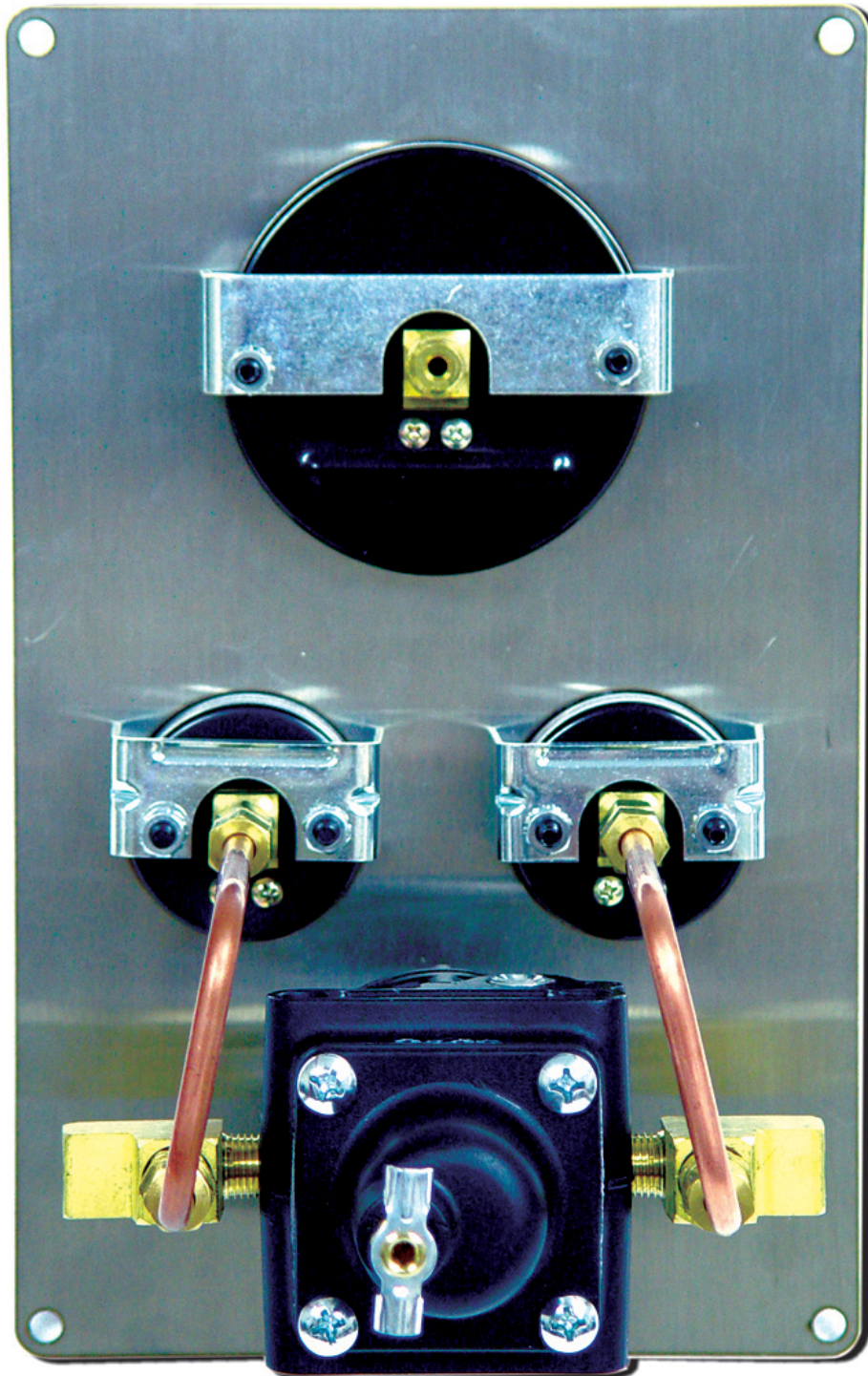
Type RCP-2 Panel Rear View (Actual Size: 7 1/4" wide x 11 1/2" high x 8" deep)
